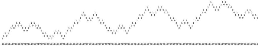
Fig. 3. Typical solution curve for \psi_{2,5}^{177} . This is the largest satisfiable formula for W(2, 5) . For both figures, the solution is shown as a sequence of 0's and 1's representing an assignment of values to variables in increasing order of index, from left to right. The top of each curve rises one unit for every 1 encountered and drops one unit for every 0 encountered when traversing the solution from left to right
