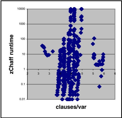
Fig. 4. \frac{\#clause}{\#var} vs zChaff I runtime
