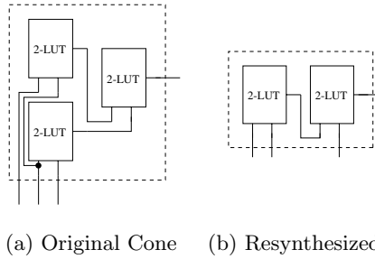
Fig. 4. Resynthesis of three-input cone of logic
