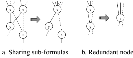
Fig. 2. Reduction Rules
