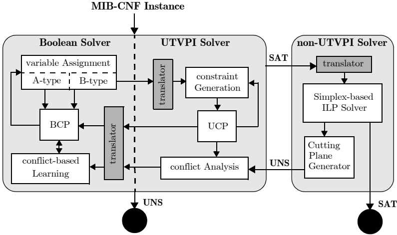
Fig. 2. Overall Architecture of the MIB-CNF Solver
