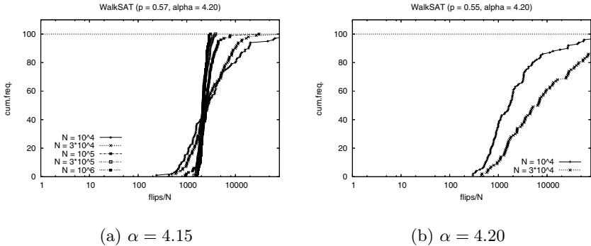
Fig. 3. Solution time distributions for WalkSAT at \alpha = 4.20 , p = 0.57 and p = 0.55
