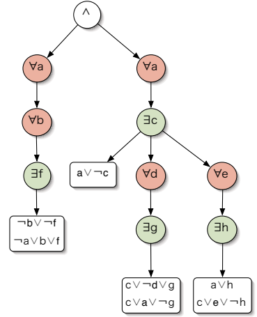
Fig. 1. A quantifier tree for (1)
